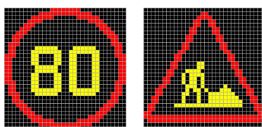
Figure M.7 — Example of VMS using (32 × 32) elements with colour inversion
