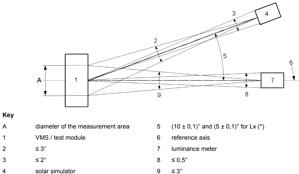
Figure 4 — Side elevation of the set-up for the measurement of luminance and luminance ratio
